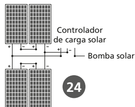
PANEL SOLAR: 4 x 340W
