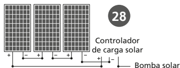
PANEL SOLAR: 3 x 550W
