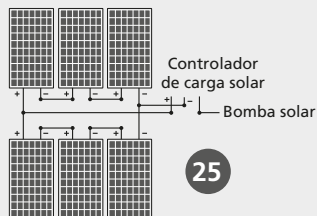
PANEL SOLAR: 6 x 265W
